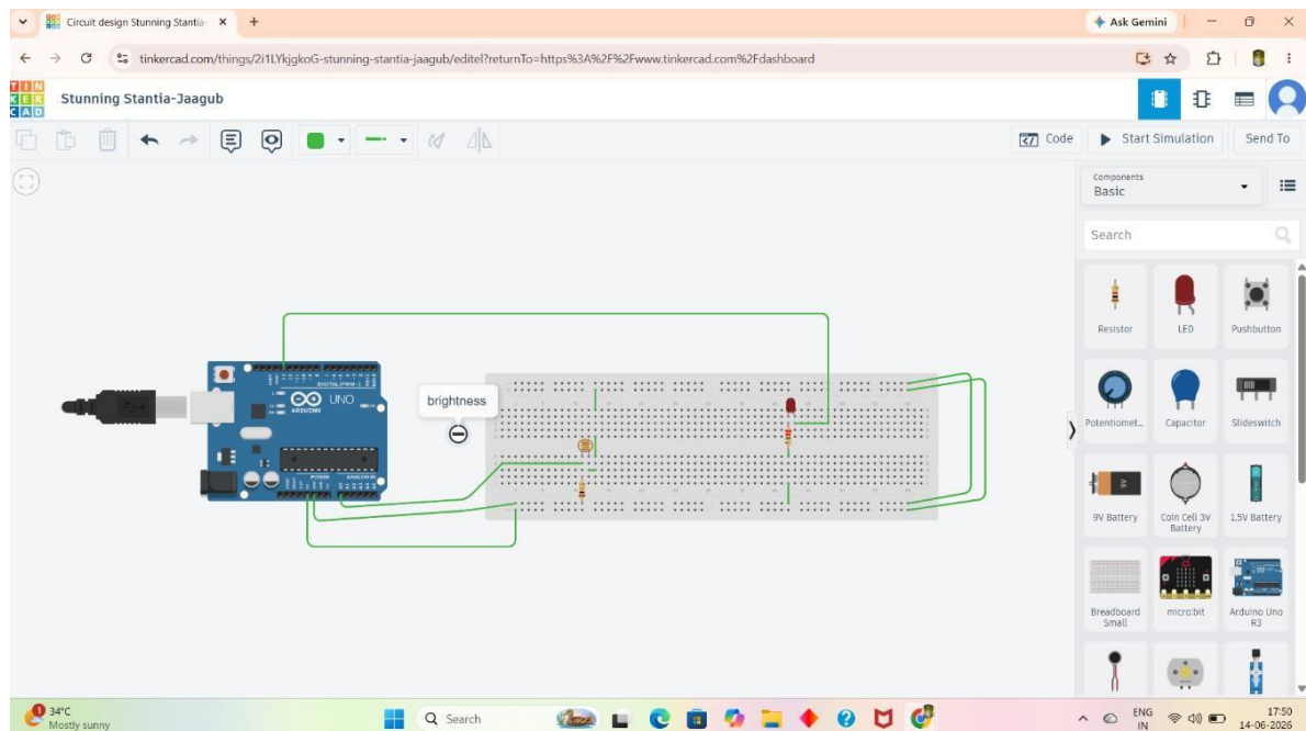
Figure 2: Complete Tinkercad Circuit.
