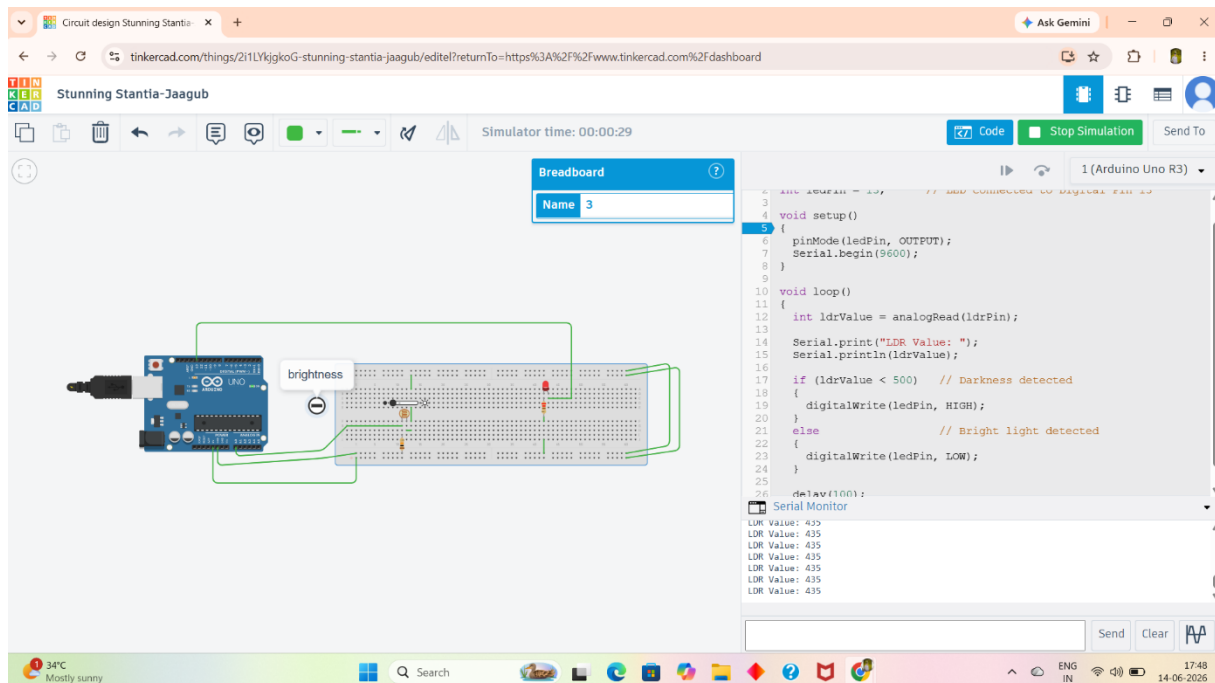
Figure 4: LED turns ON during darkness.
